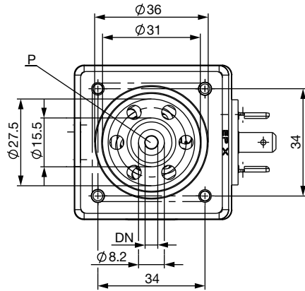
Sub-base body
