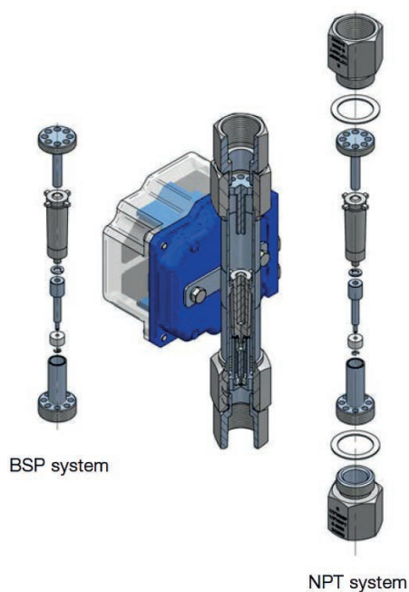
Damping system for M-21 1/2" and 3/4"
