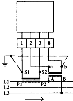
LSC 96KD/PFQ 13 3-phase, 3-wire balanced load.
